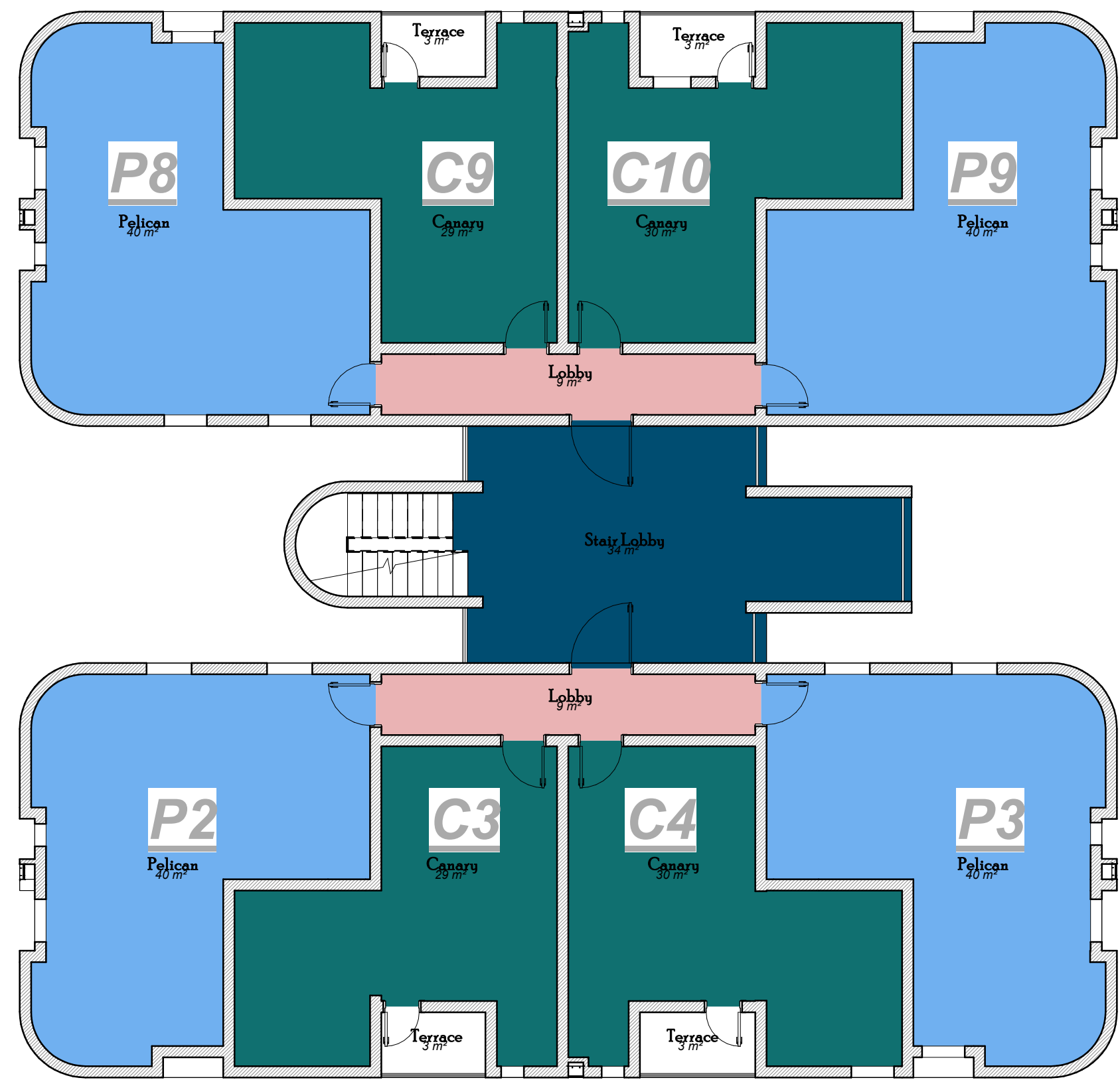
2 2 FIRST FLOOR PLAN 1 : 100
