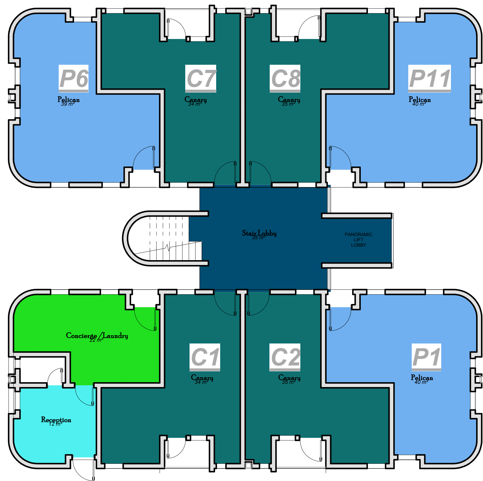
1 1 GROUND FLOOR PLAN 1 : 100
